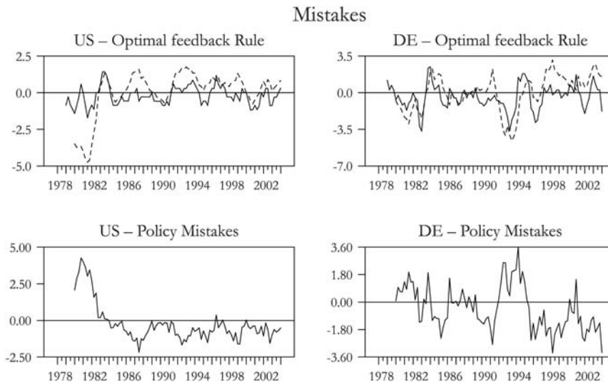
Figure 5. OFR (dashed lines) vs actual hours (solid lines) and the policy mistakes
