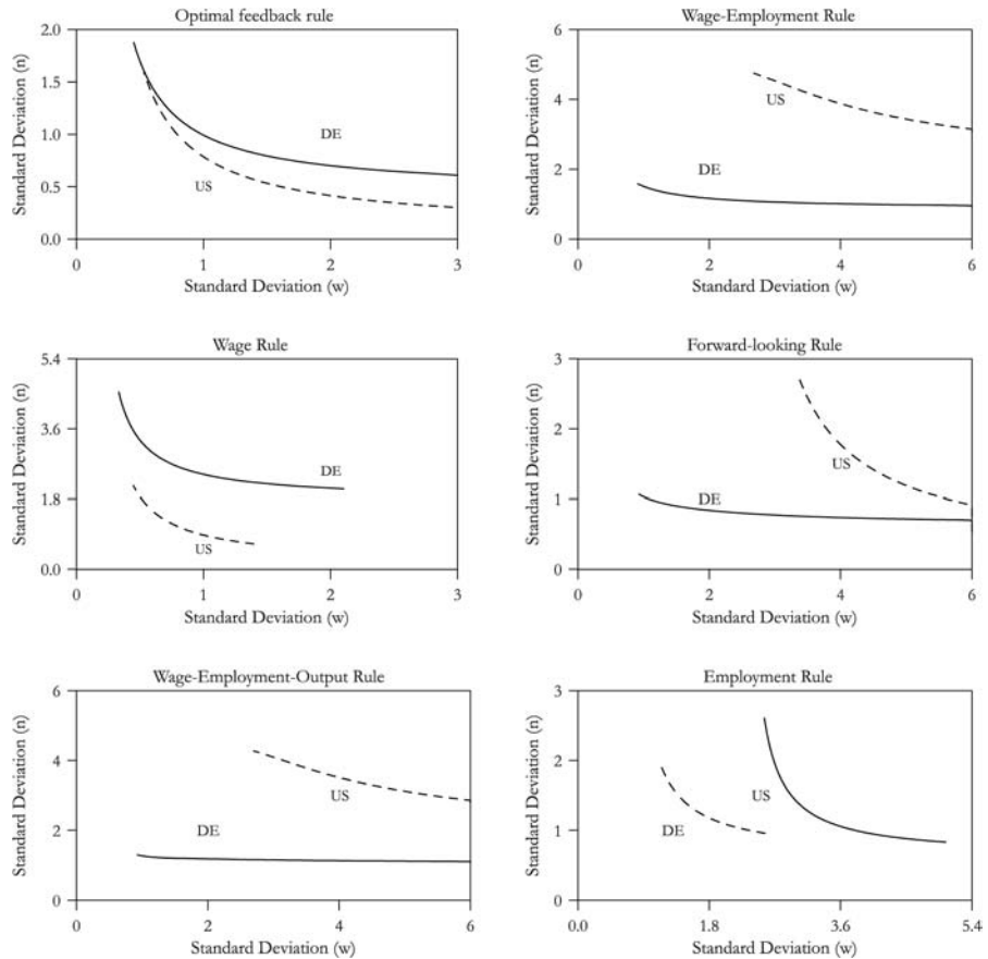
Figure 6. The efficiency frontiers for the six rules in Germany and the USA
